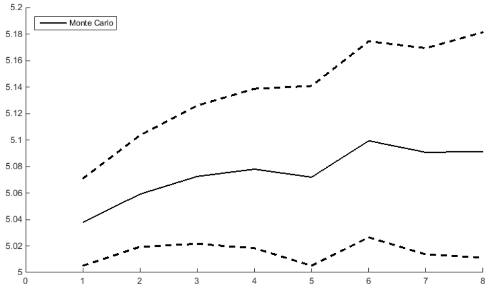
Figure 15: Using a Monte Carlo Simulation for 8 quarters (2 years)
